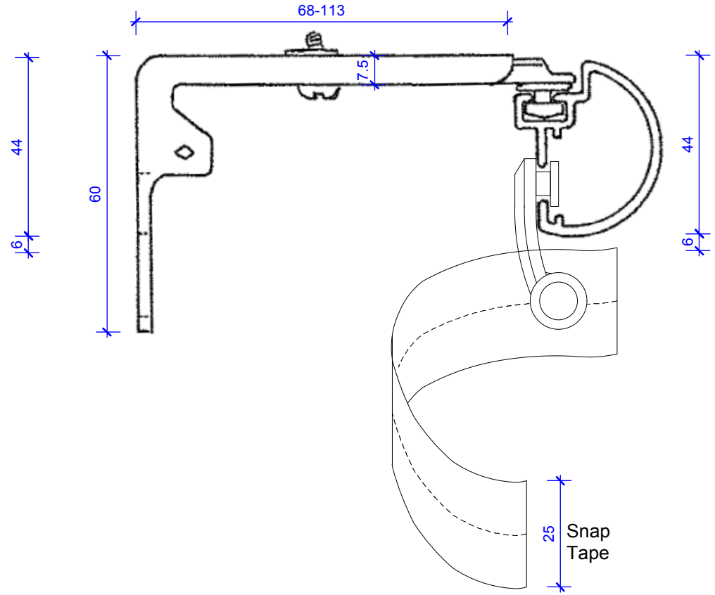
SERIES 66 DOMESTIC TRACKING S-FOLD Single Bracket
