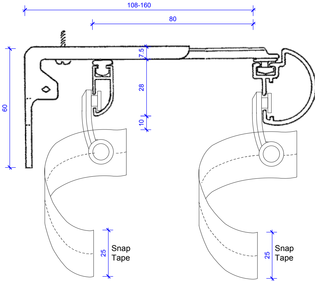
SERIES 66 DOMESTIC TRACKING S-FOLD Double Bracket
