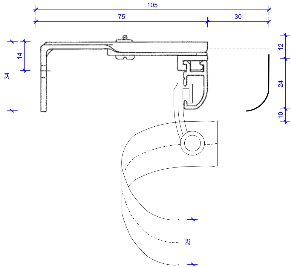
SERIES 73 DOMESTIC TRACKING S-FOLD Single Centre Support Bracket No 7355
