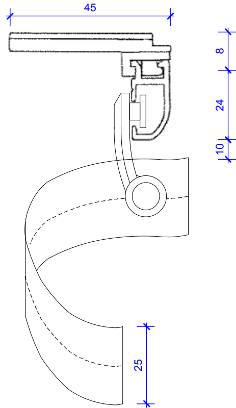
SERIES 73 DOMESTIC TRACKING S-FOLD Ceiling Fix Bracket No 7353
