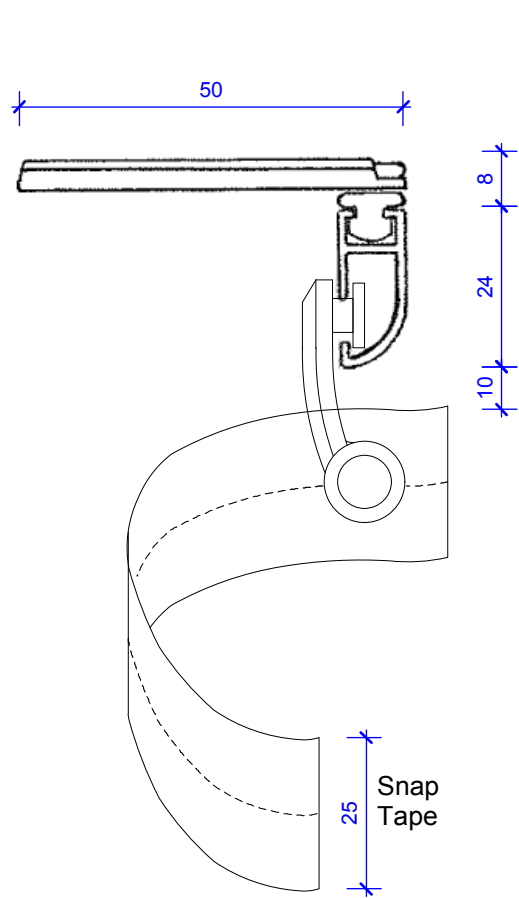
SERIES 79 DOMESTIC TRACKING S-FOLD Ceiling Fix Bracket No 7953
