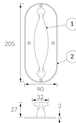
112197 729 Handle on 90 x 205mm Radius Plate
