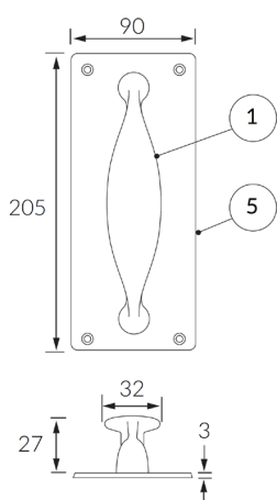
116237 729 Handle on 90 x 205mm Square Plate
