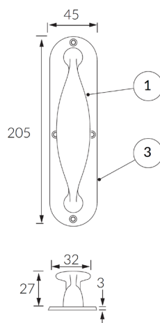
114180 729 Handle on Narrow Radius Plate 45 x 205mm
