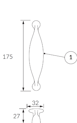
116236 729 Handle without Backplate
