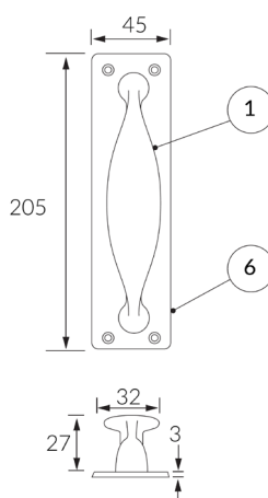
116238 729 Handle on Narrow Square Plate 45 x 205mm
