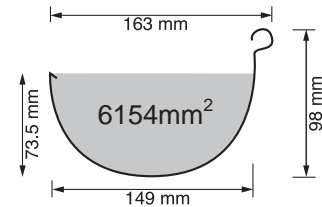
Half Round Slotted
