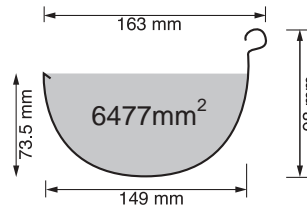
Half Round Unslotted
