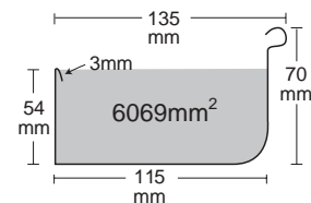
Old Style Quad
