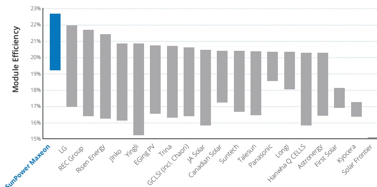
Commercialised Solar Panel Efficiencies 11
