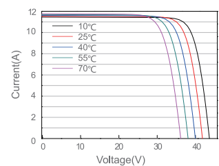
Current-Voltage Curve JAM60S20-380/MR/1000V
