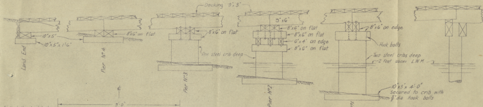
End Elevation of Piers
