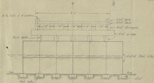
Front Elevation Pier N°1.
