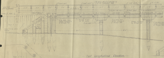
Part Longitudinal Elevation.
