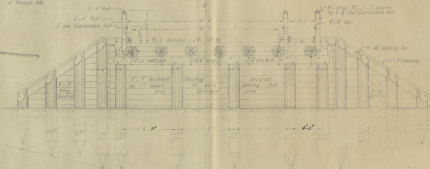
Sectional Elevation on C-D
