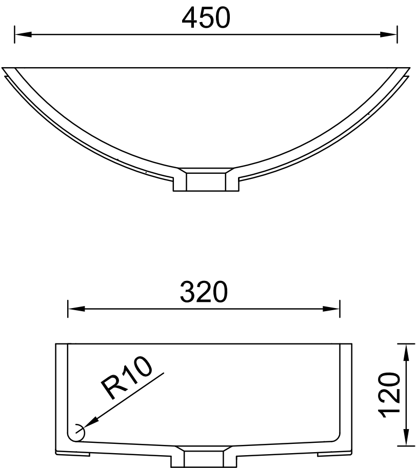
CROSS-SECTION
