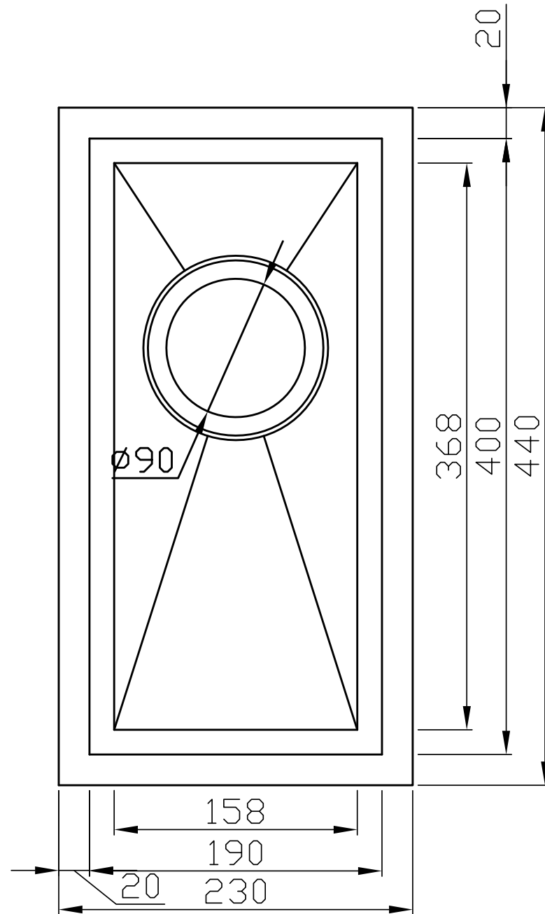
Top View
