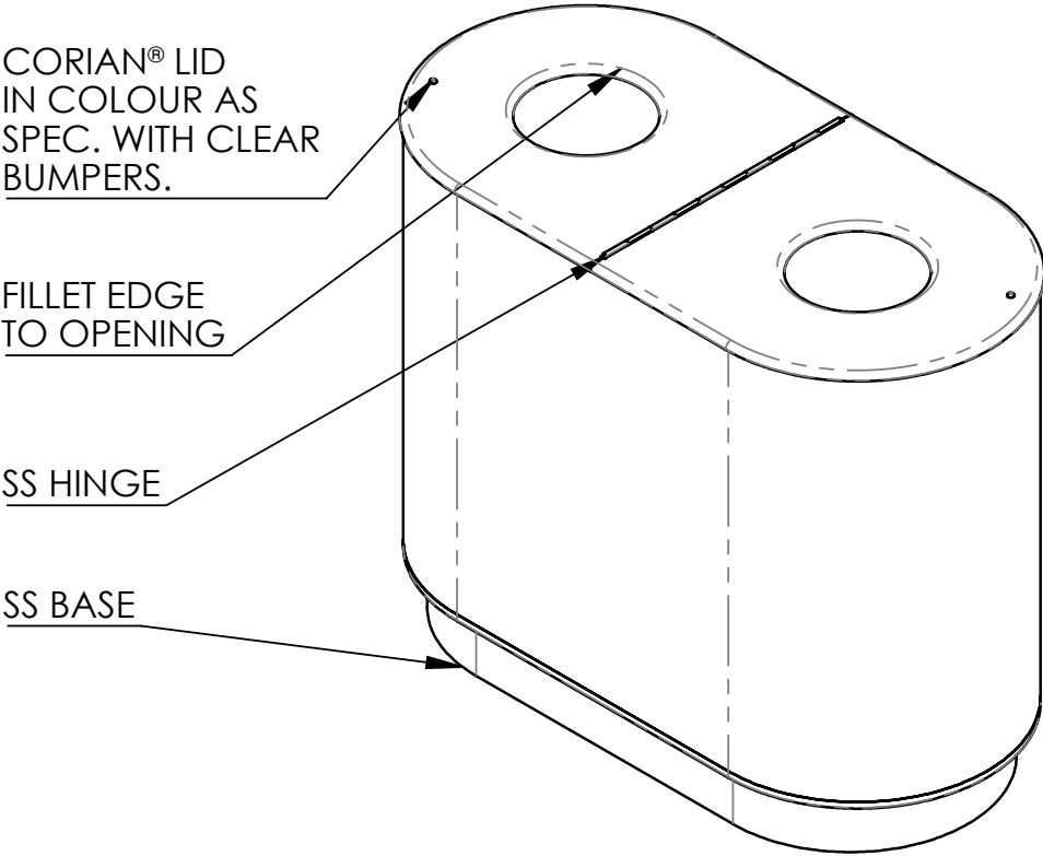
ISOMETRIC VIEW
