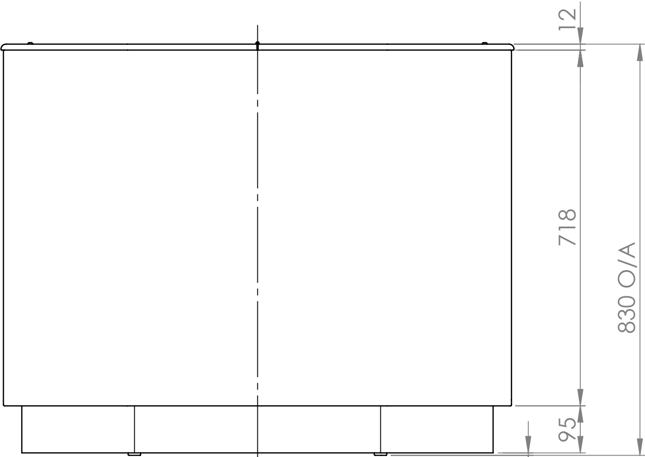
FRONT VIEW
