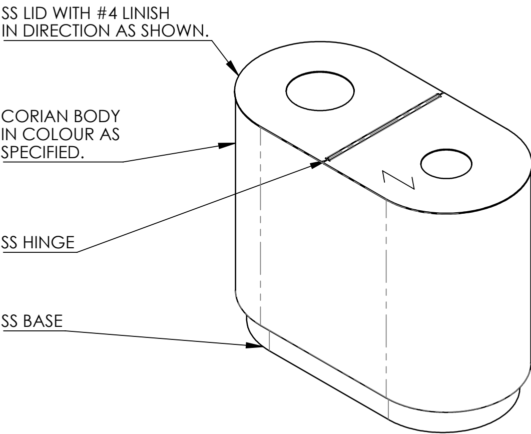
ISOMETRIC VIEW
