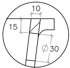
DETAIL C SCALE 2: 5
