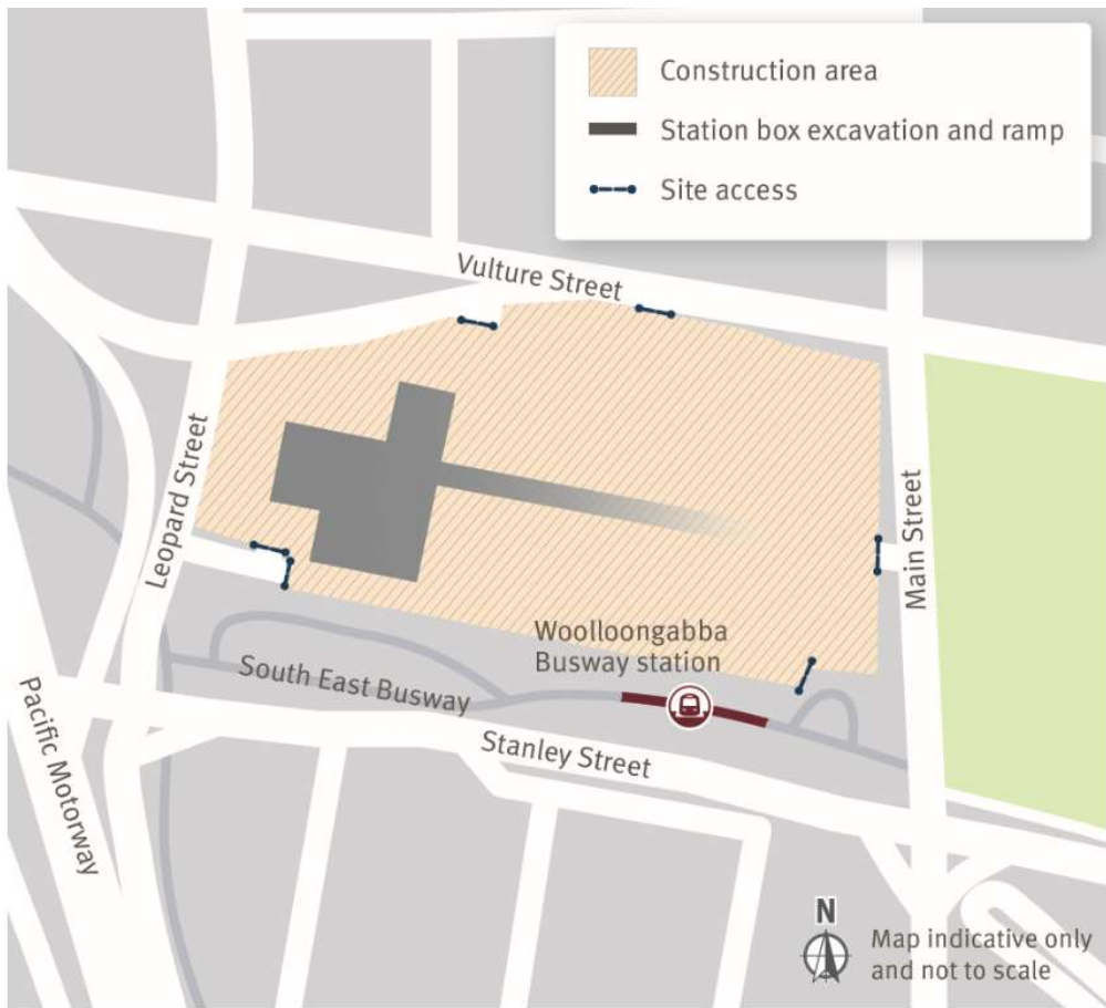
Image 1: Updated Woolloongabba site, showing access points for construction vehicles
