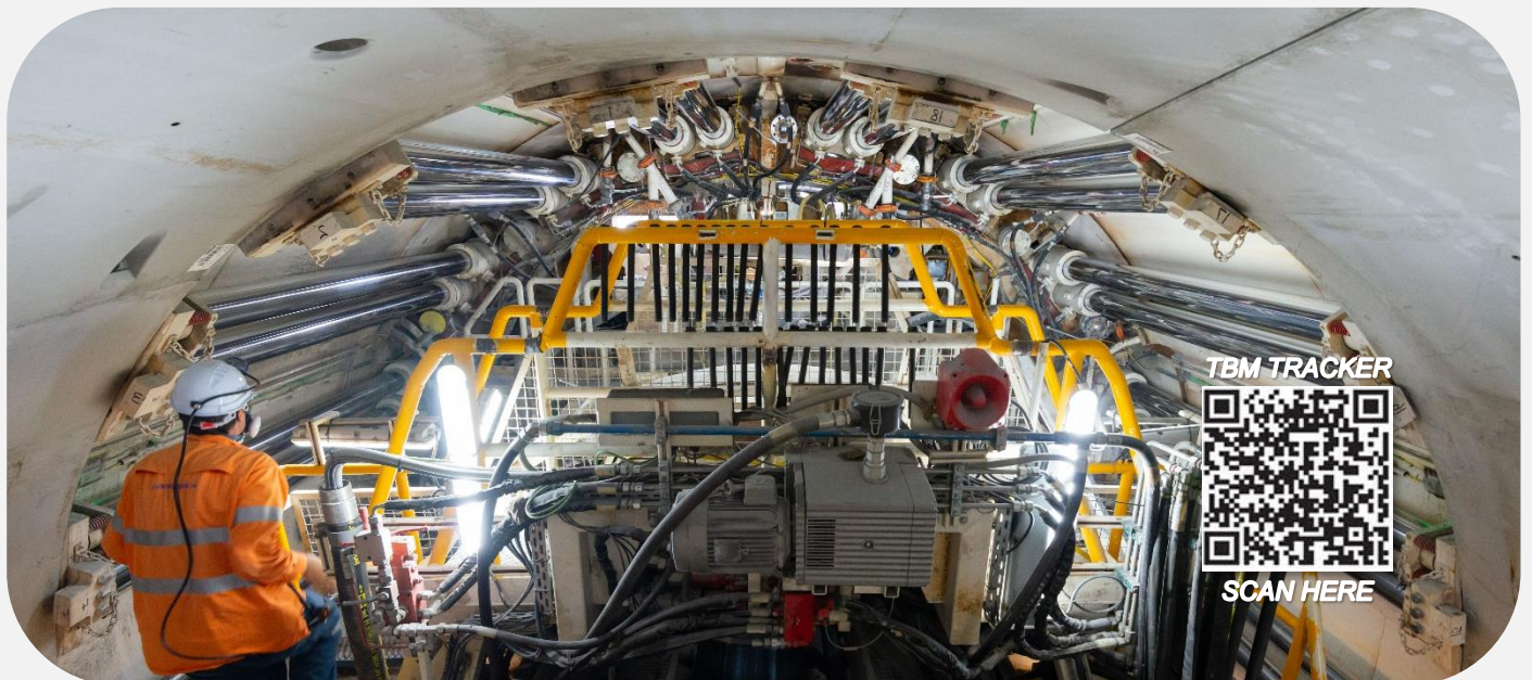
The view from inside TBM Else
