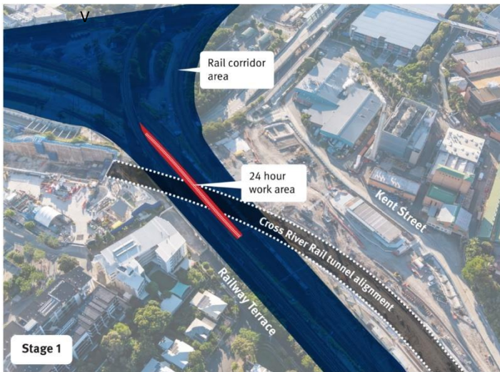
Stage 1: Extended 24 hour rail corridor works
