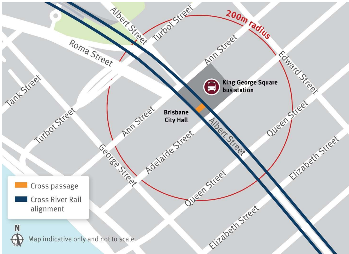
Location of cross passage beneath King George Square
