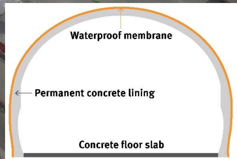
Cross-section of permanent tunnel lining
