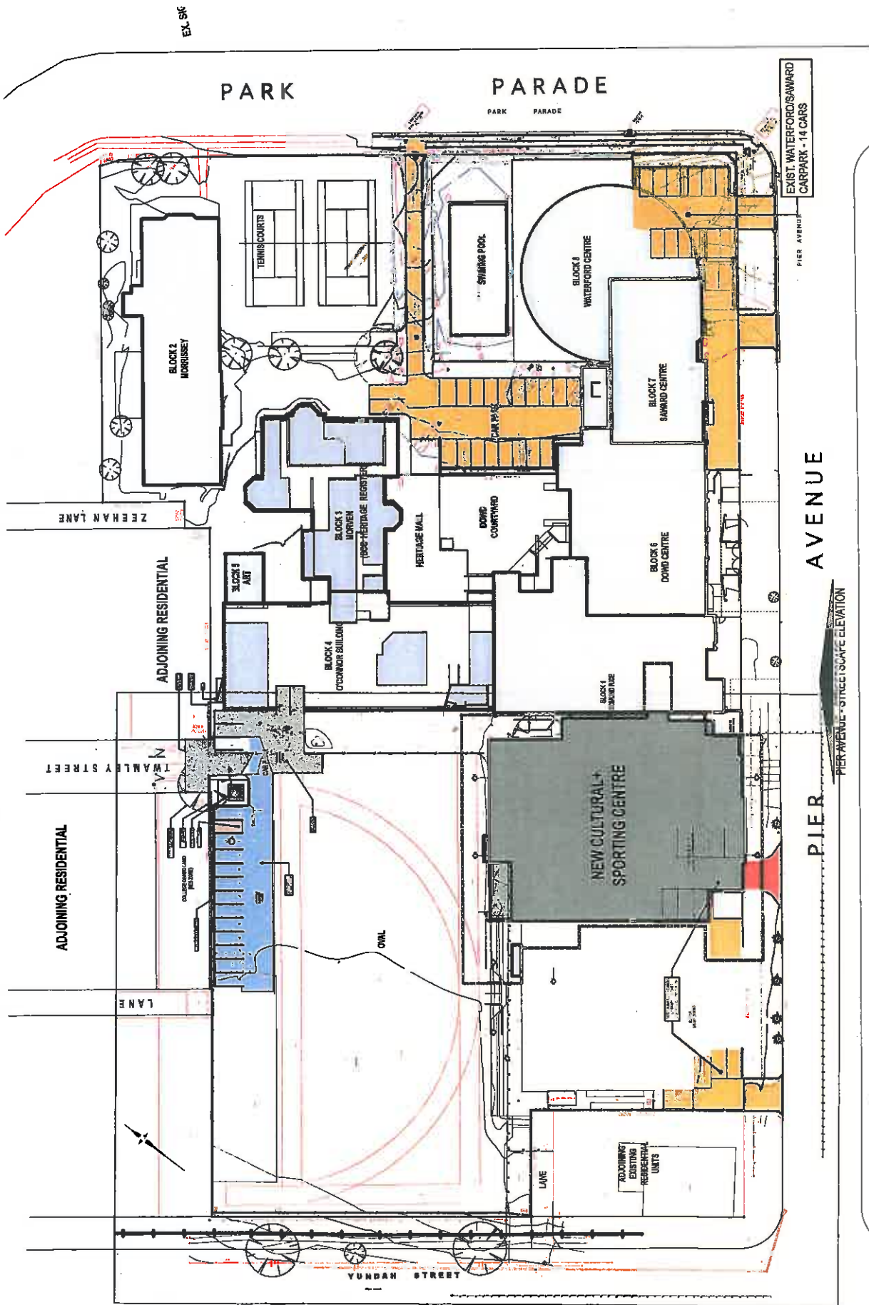
OVERALL SITE PLAN 1:500
