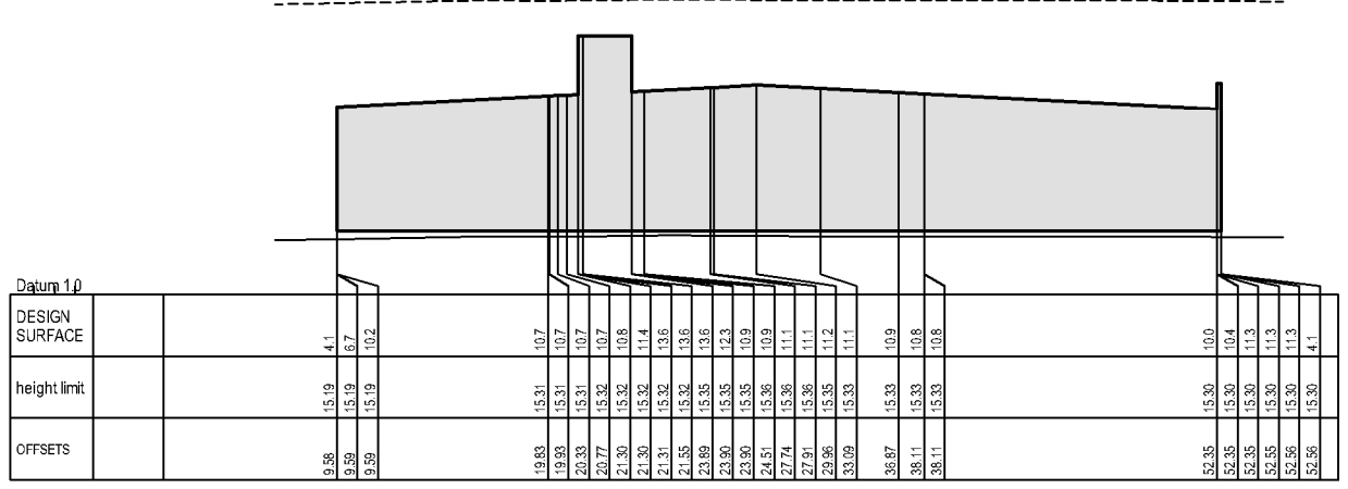
SECTION C-C
