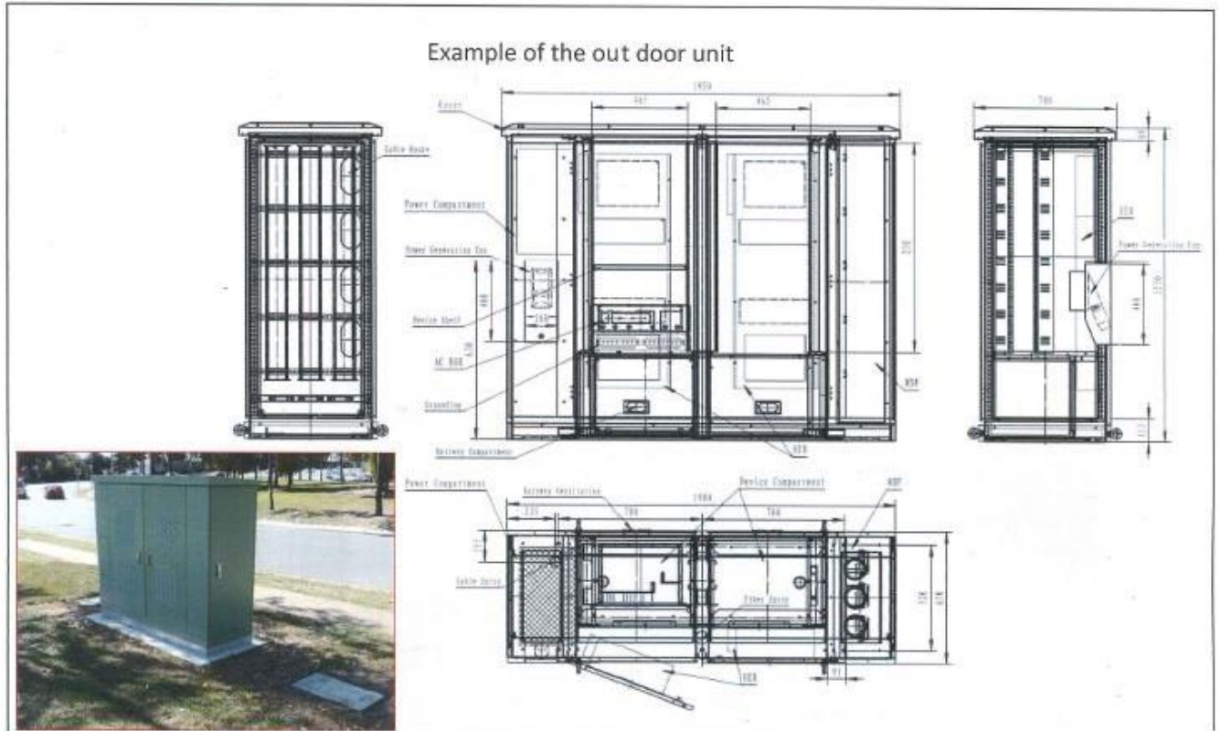
Fig.2. Proposed Telecommunication Equipment.
