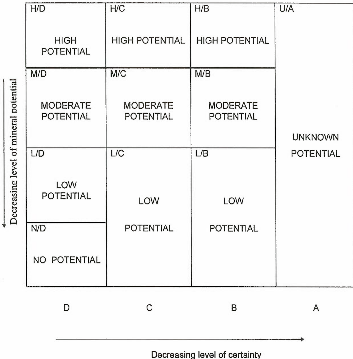
Figure 3: Relationship between Levels of Resource Potential and Levels of Certainty
