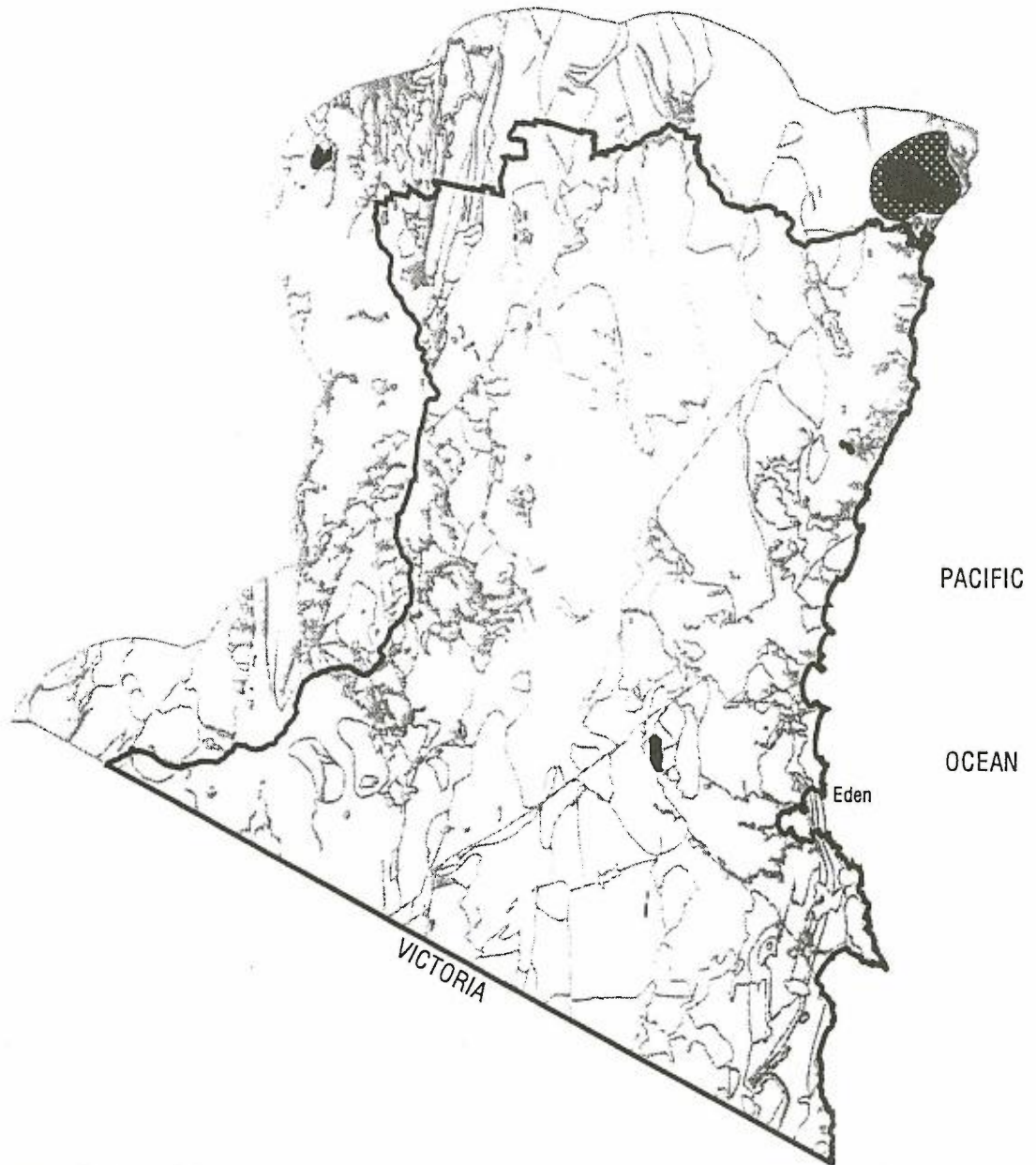
Figure 6: Mineral potential tracts for gold deposits associated with alkaline rocks
