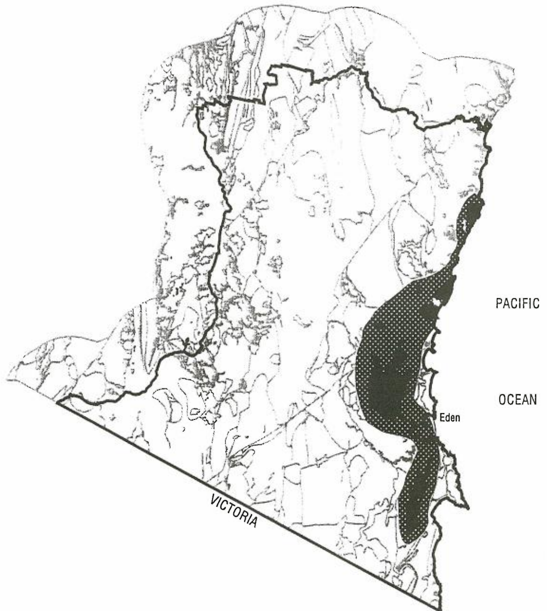
Figure 5: Mineral potential tracts for epithermal gold-silver and pyrophyllite deposits
