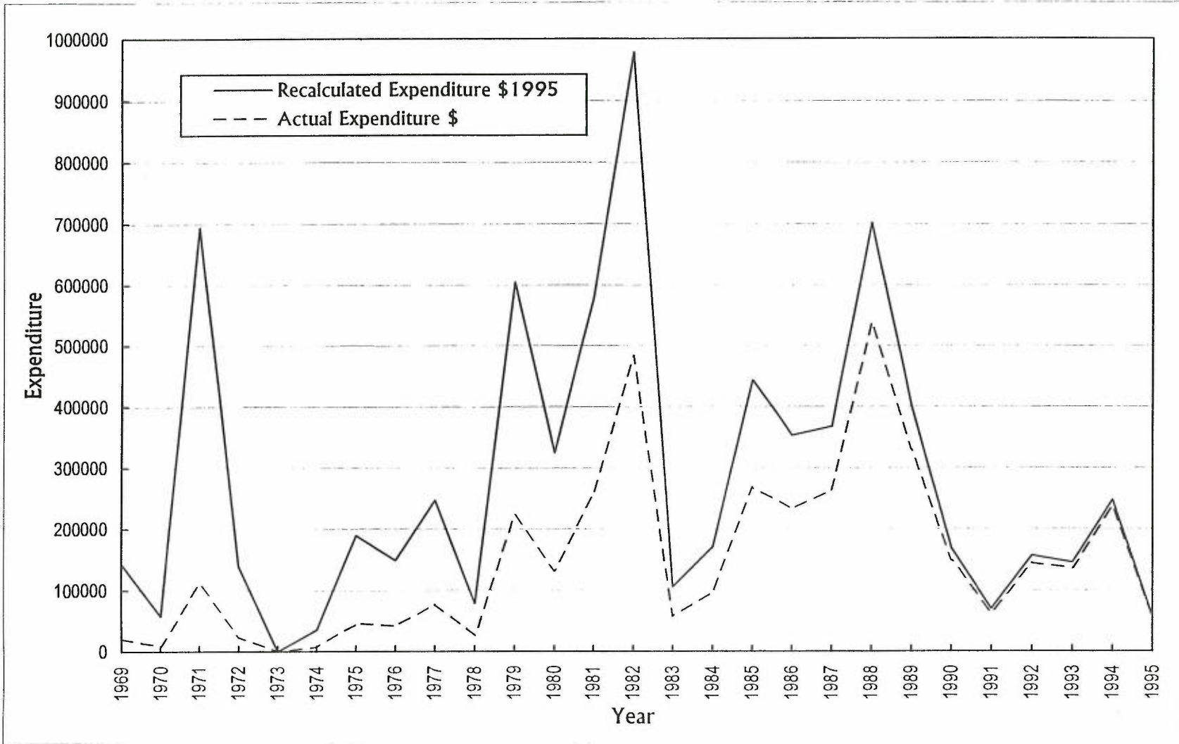
Figure 1: Exploration expenditure in the Eden region during 1969 - 1995.
