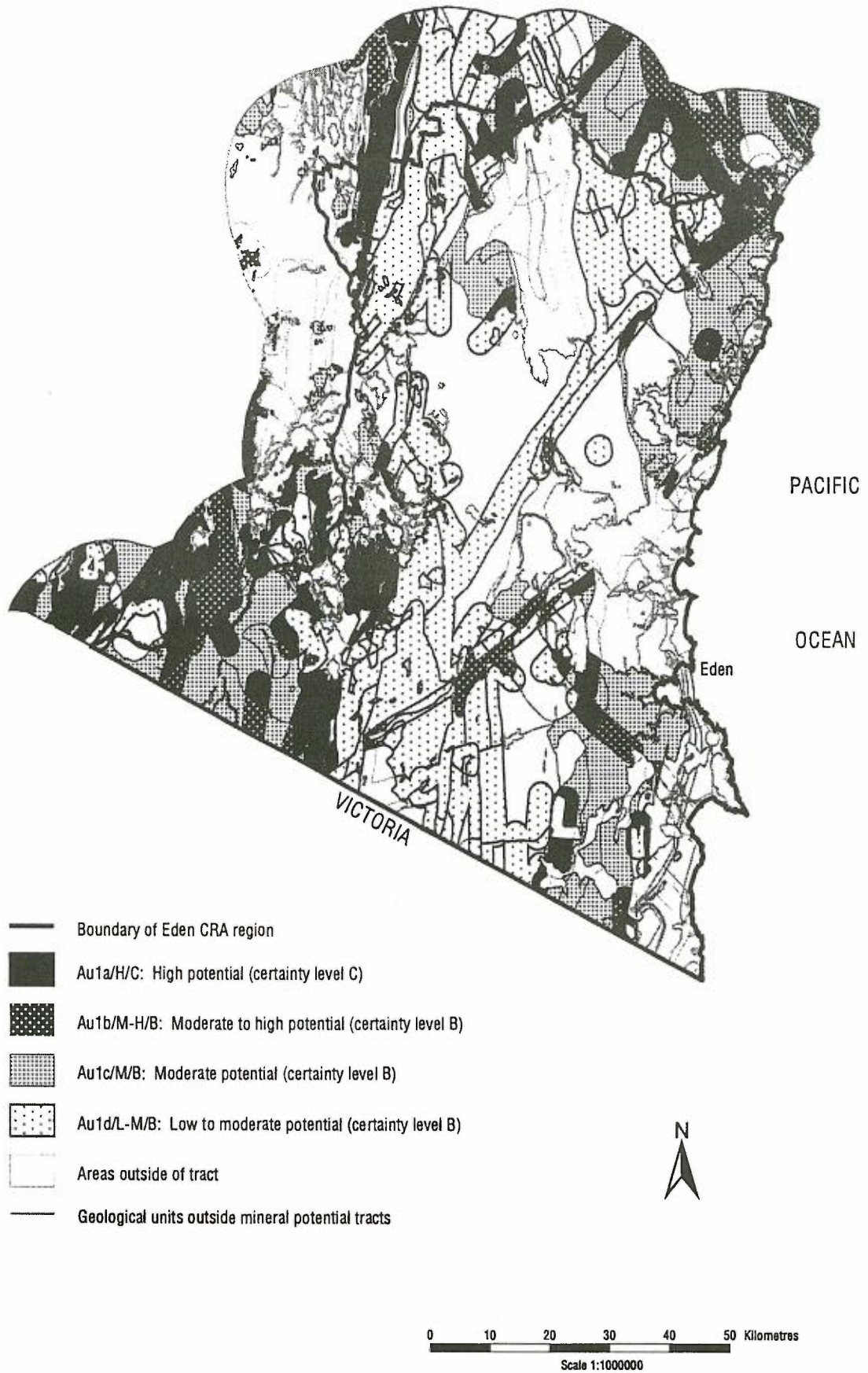
Figure 4: Mineral potential tracts for slate belt gold deposits
