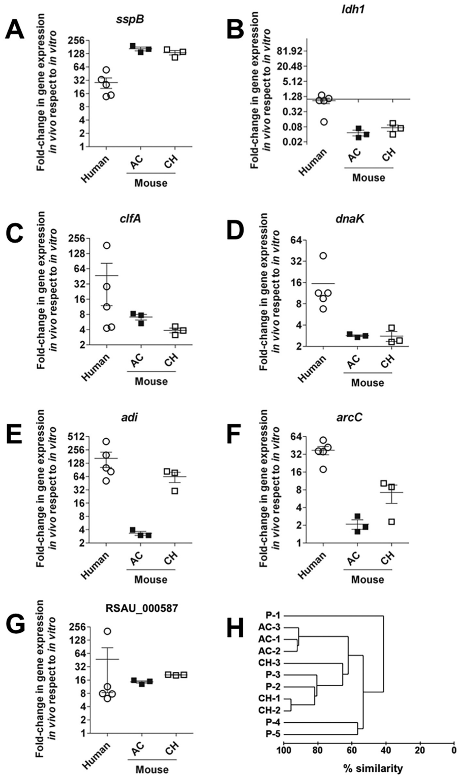
FIG 5 Confirmation of selected S. aureus in vivo -expressed genes in clinical samples by qRT-PCR. Changes (fold) in expression of sspB (A), ldh1 (B), clfA (C), dnaK (D), adi (E), arcC (F), and the gene encoding the manganese ABC transporter (RSAU_000587) (G) in S. aureus in infected human tissue (circles) were determined by qRT-PCR, and those in murine bones (squares) were determined by RNA-Seq. The expression of the respective gene by S. aureus grown in vitro in rich medium was used as a reference to calculate the changes. Each circle represents one individual patient, and each square represents one independent experimental set in the murine system, with black squares representing AC infection and white squares CH infection. (H) Hierarchical clustering dendrogram showing the change (fold) in gene expression data determined by Bray-Curtis similarity scores. P-1 to P-5, individual patients; AC-1 to AC-3, individual data sets from murine AC bone infection; CH-1 to CH-3, individual data sets from murine CH bone infection.
