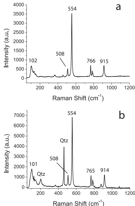
FIGURE 4. Comparison of Raman spectra of synthetic and natural Rb pentaborate tetrahydrate. (a) Synthetic Rb pentaborate tetrahydrate and (b) natural ramanite-(Rb) in an inclusion in graphic quartz from the Elba pegmatite. Peak labels (in \text{cm}^{-1} ) refer to the diagnostic bands. Qtz = strong Raman bands of the quartz matrix.
