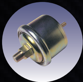
Sender 545-20 Oil pressure (electric) 1/8" NPT
