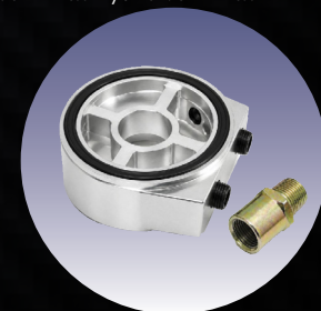
Sandwich Plate 547-49 Oil pressure & Temp Adaptor 13/16" -16"
