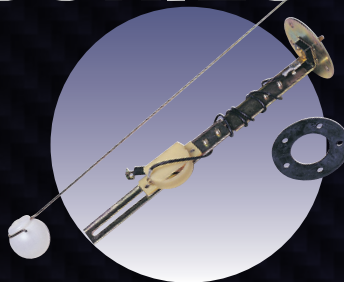
Sender 545-40 fuel level (adjustable) for 523-06/524-06/535-06/537-06 gauges
