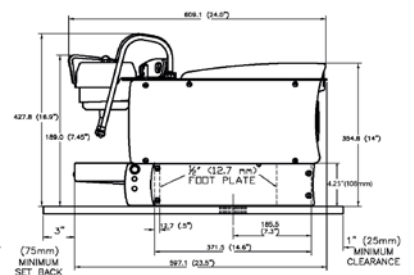
RIGHT HAND END VIEW
