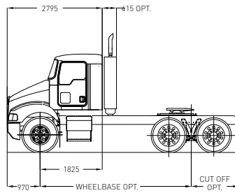
T359 DAY CAB
