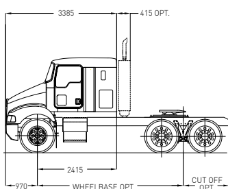
T359 28" IT SLEEPER
