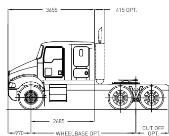
T359 36" RECESSED BACK FLAT ROOF SLEEPER
