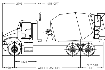
T359A DAY CAB 6x4
