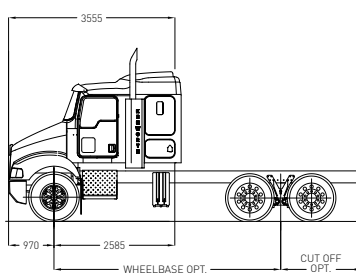
T359 36" RECESSED BACK MID ROOF SLEEPER
