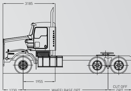
T659 DAY CAB
