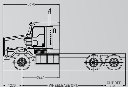
T659 28' IT SLEEPER
