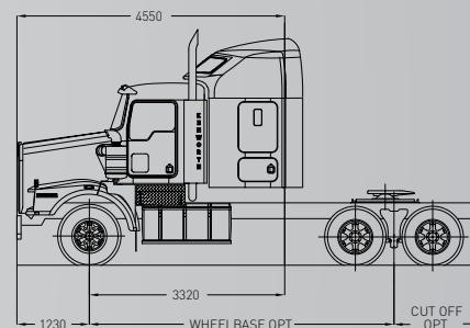
T659 1270MM AERO II ROOF SLEEPER
