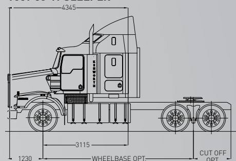
T659 50' IT SLEEPER
