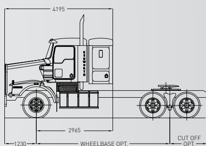
T659 915MM FLAT ROOF SLEEPER
