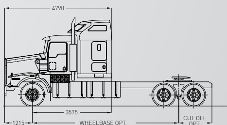
T659 1525MM AERO II ROOF SLEEPER
