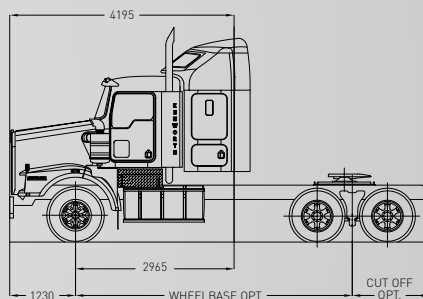
T659 915MM AERO II ROOF SLEEPER
