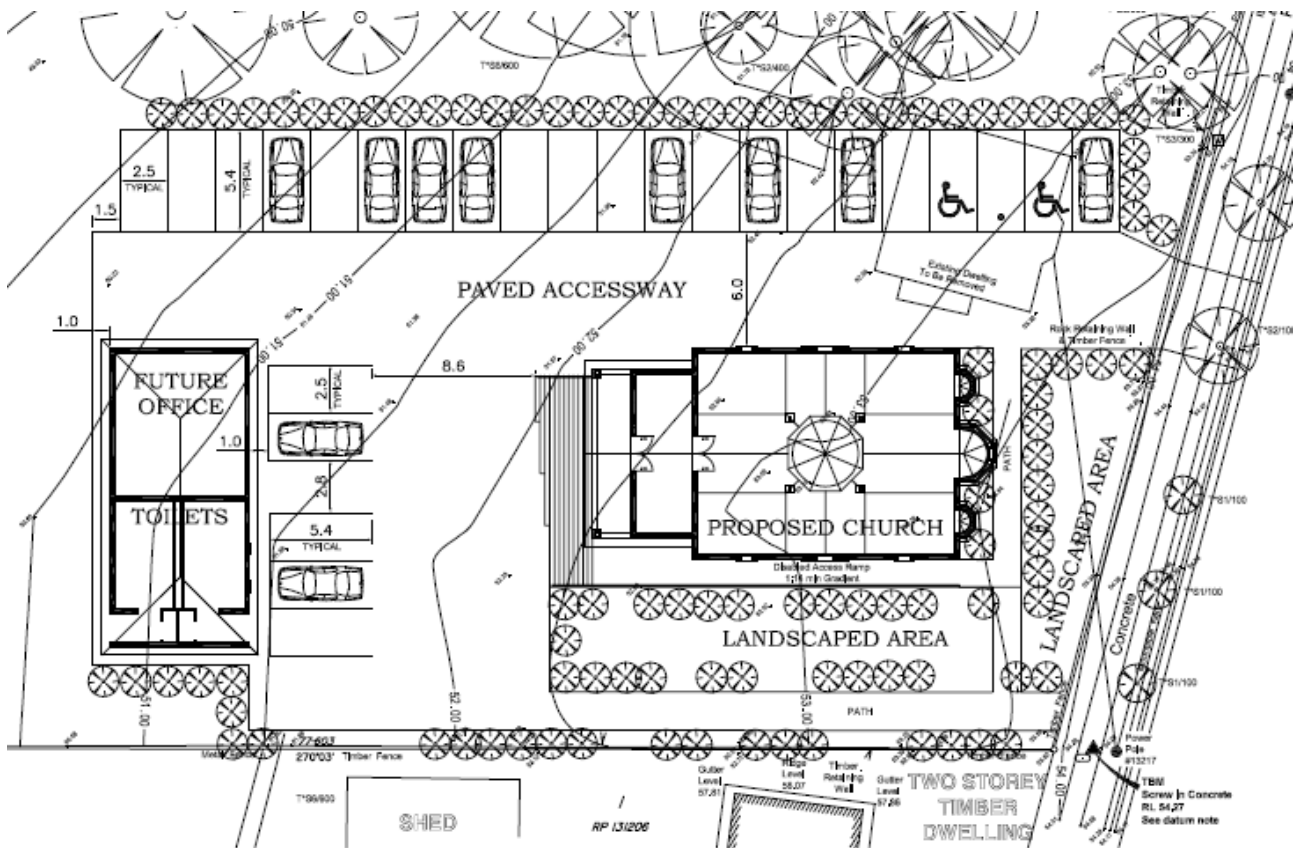
Figure 3.1 Preliminary Site Layout Plan
