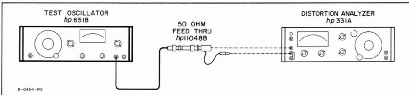
Figure 5-4. Distortion Check
