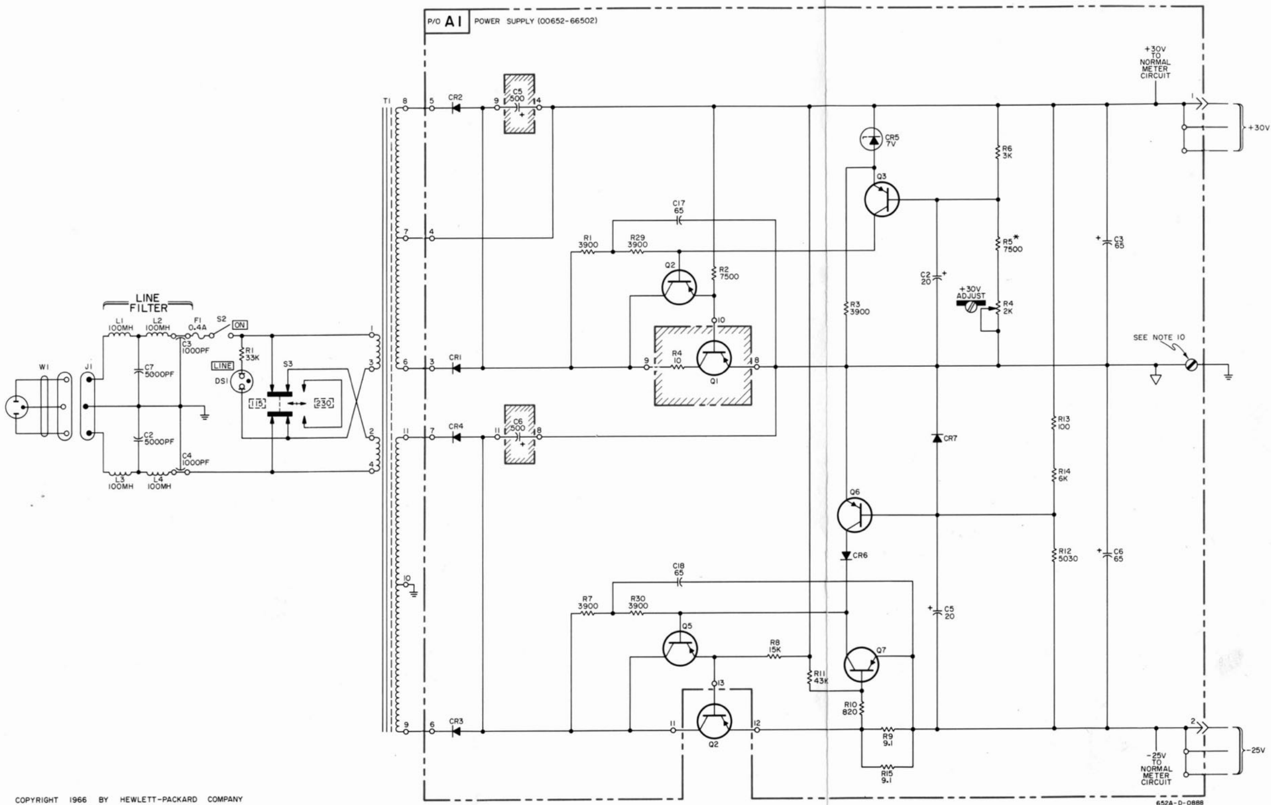
Figure 6-3. Monitor Circuit and Power Supply
