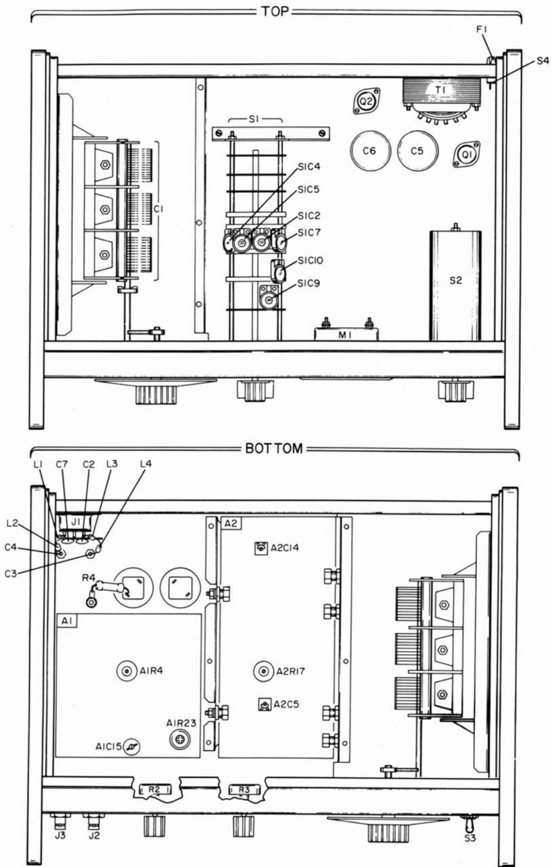
Figure 5-7. Location of Internal Adjustments
