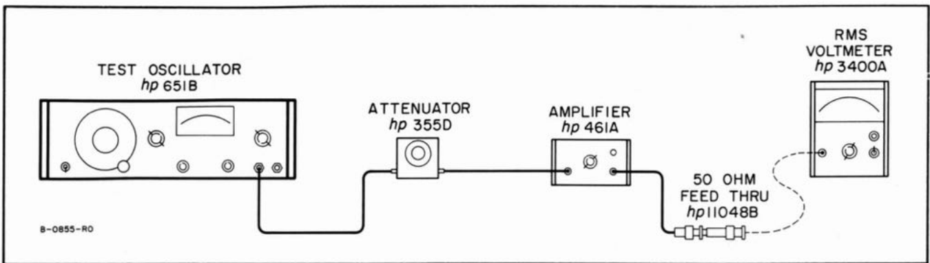
Figure 5-5. Attenuation Check
