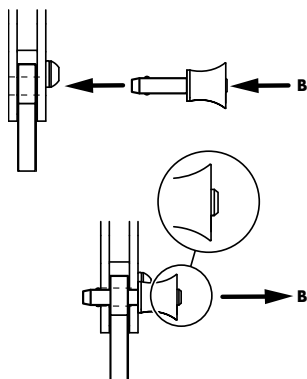
Fig. 4: Locking pins for the cabinet's Front links.
