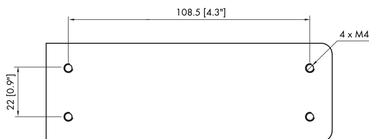
Fig. 3: Dimension of the mounting plate in mm [inch]
