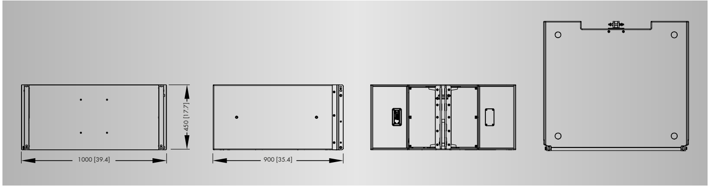
KSLi-SUB cabinet dimensions in mm [inch]
