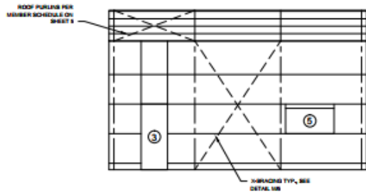
1 SIDEWALL EXTERIOR ELEVATION SCALE: 1:100
