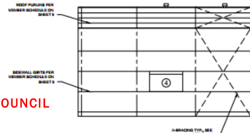
2 SIDEWALL EXTERIOR ELEVATION SCALE: 1:100
