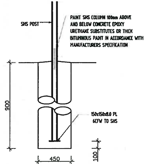
P1 FOOTING DETAIL SCALE 1:20
