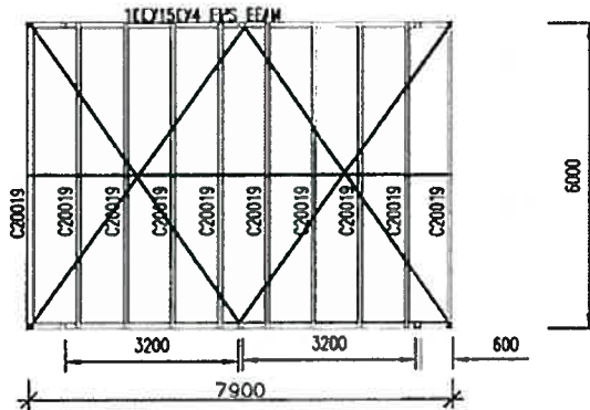
PURLIN LAYOUT PLAN SCALE 1:100
