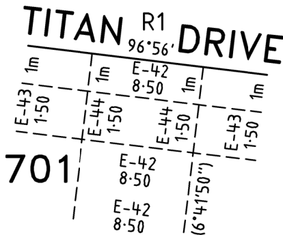
ENLARGEMENT No.3 NOT TO SCALE
