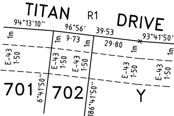
ENLARGEMENT No.4 NOT TO SCALE
