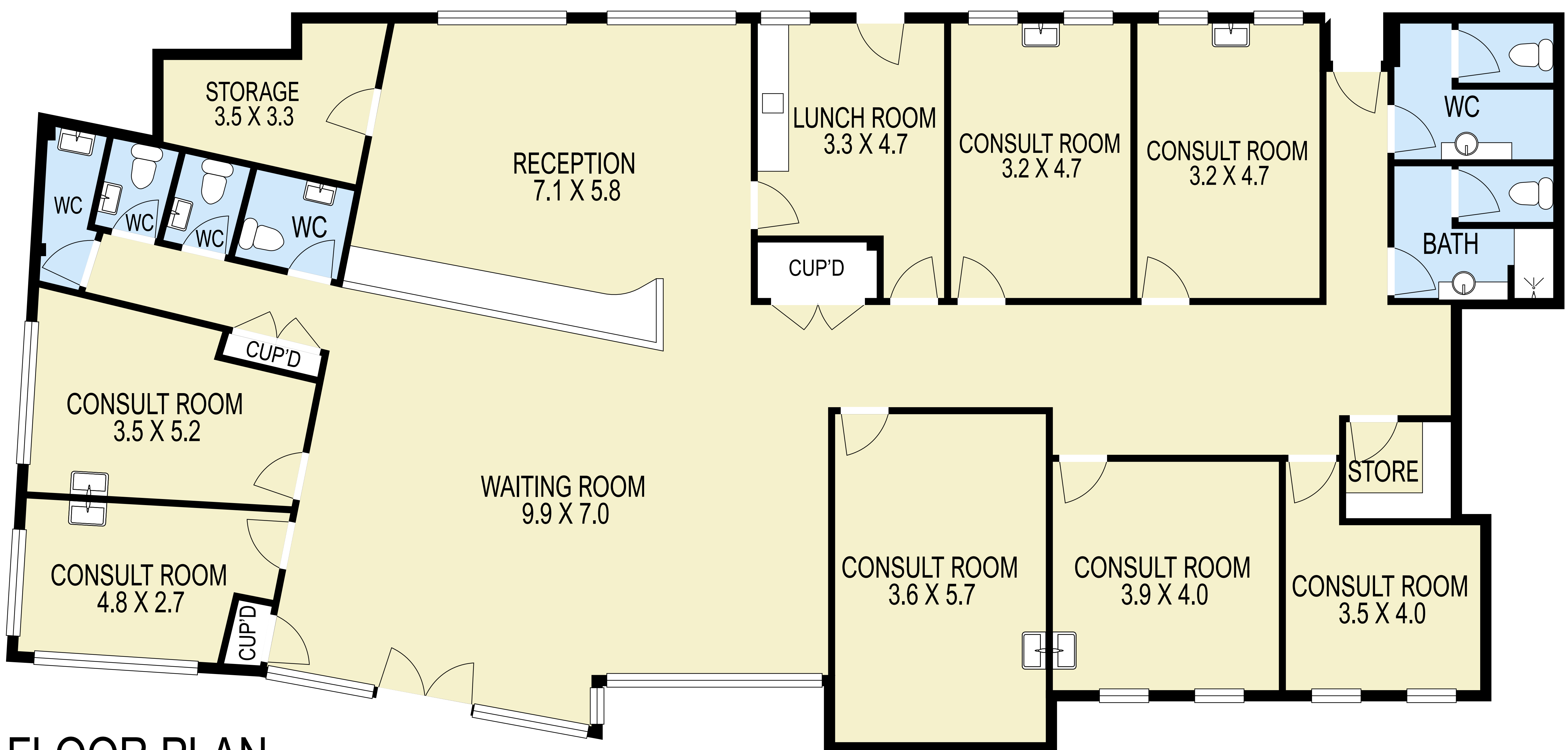
FLOOR PLAN
