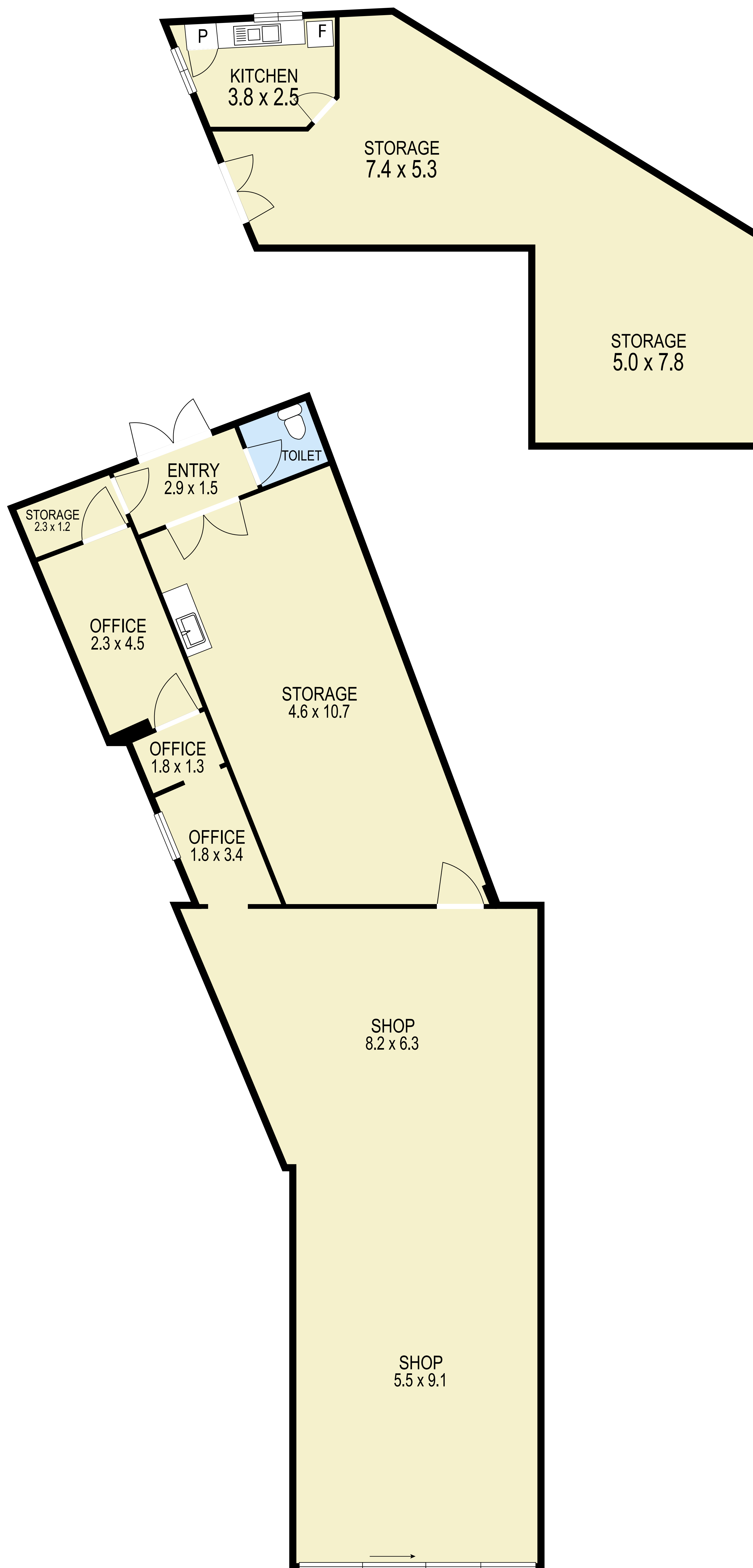
FLOOR PLAN
