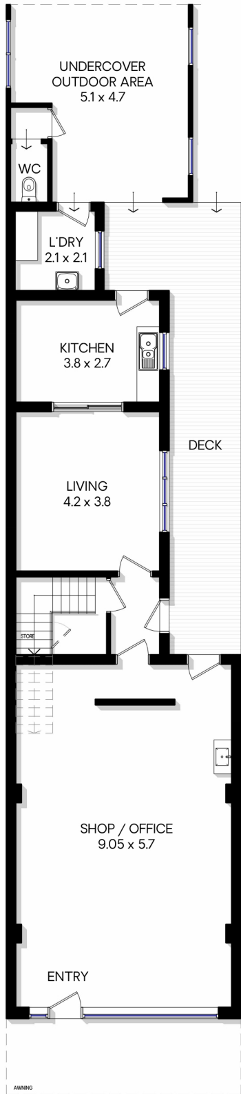
GROUND LEVEL FLOOR PLAN
