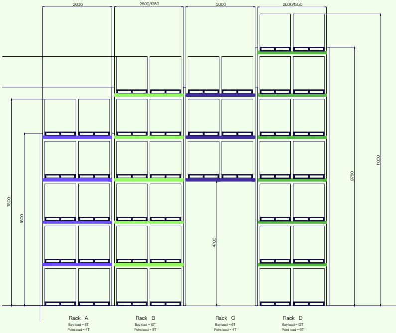
Bay elevation
