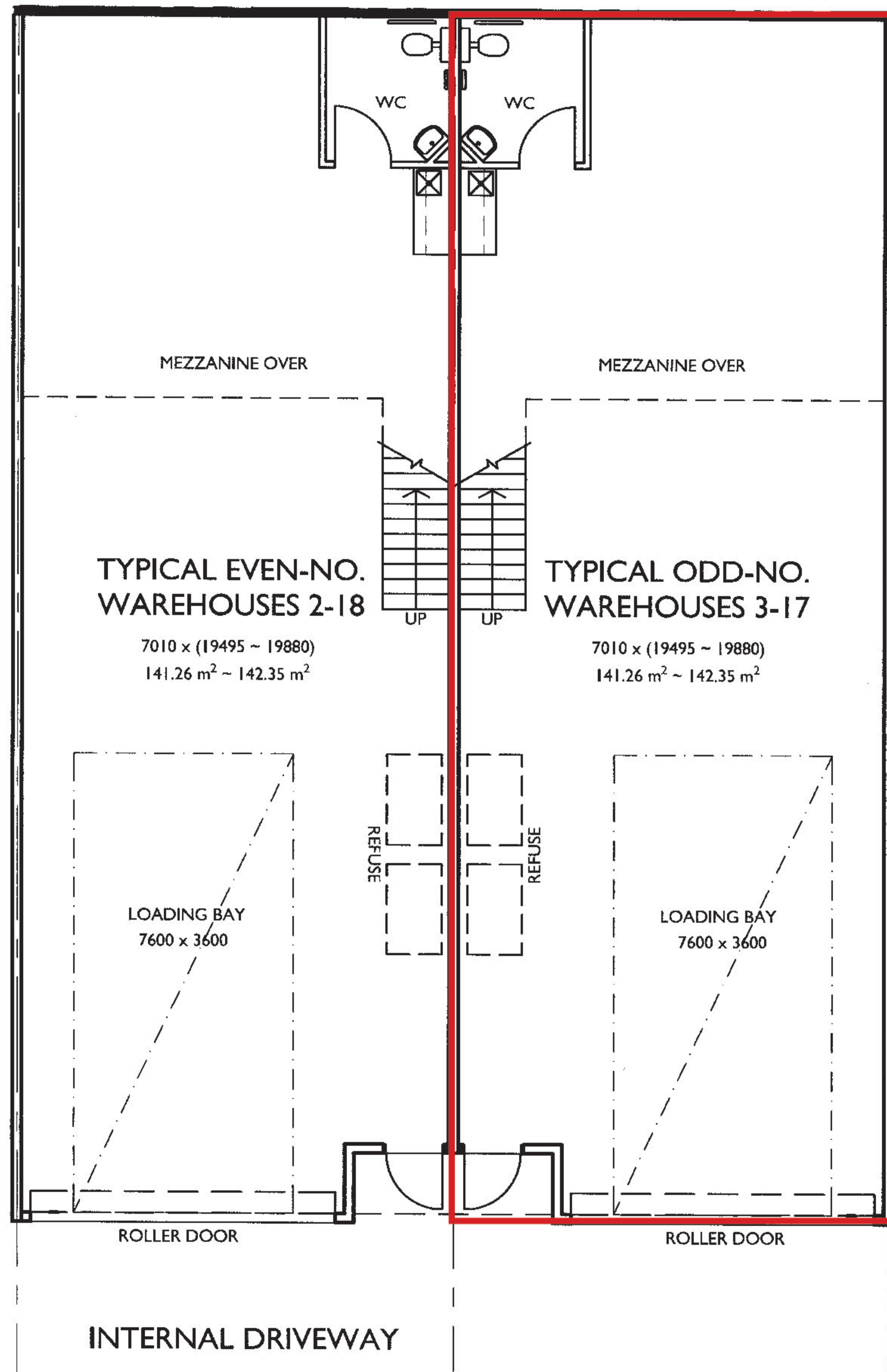
GROUND FLOOR PLAN 1:100
