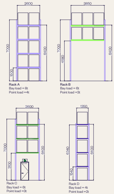
Bay elevation Scale 1:60
