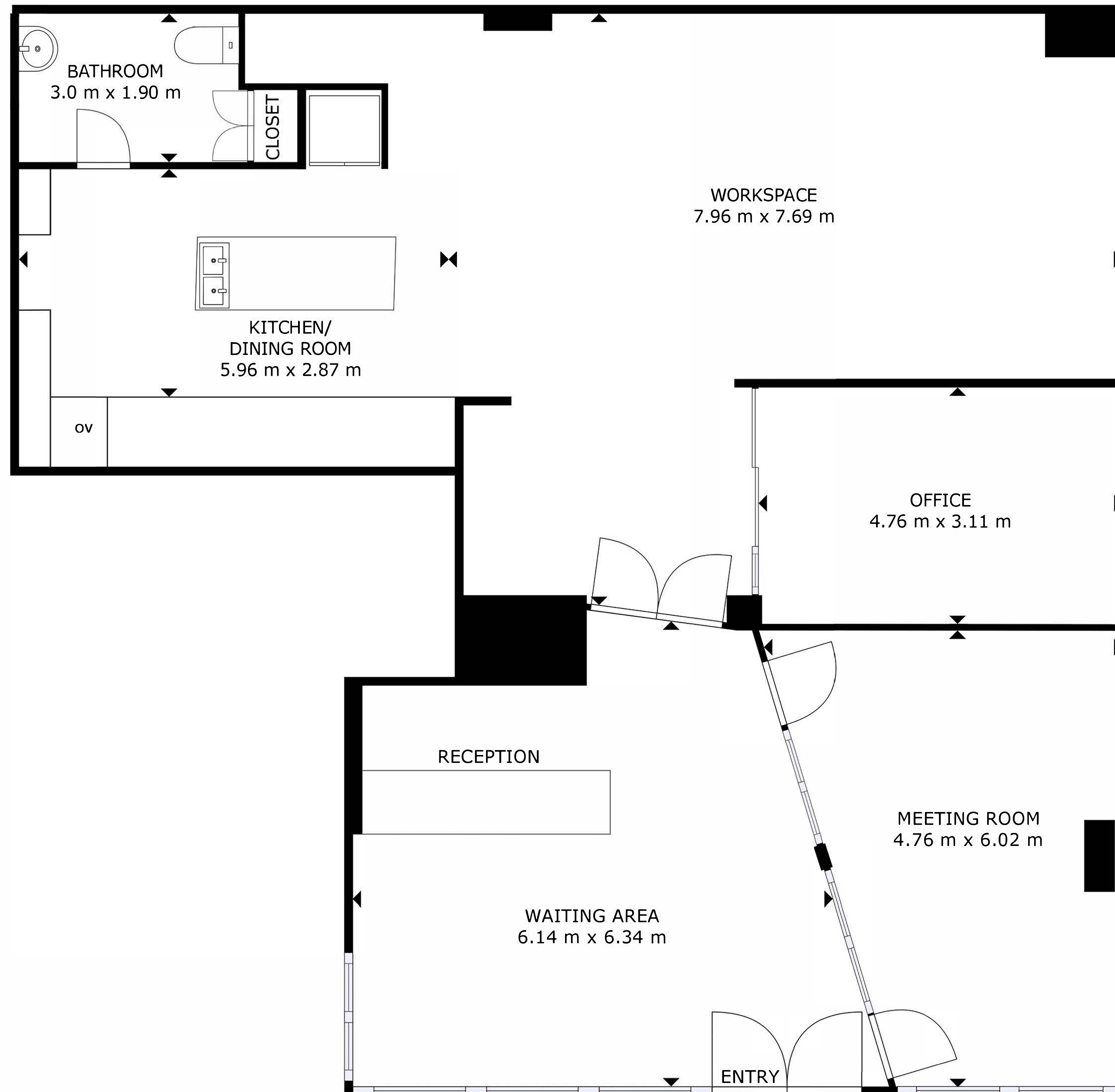
FLOOR PLAN
