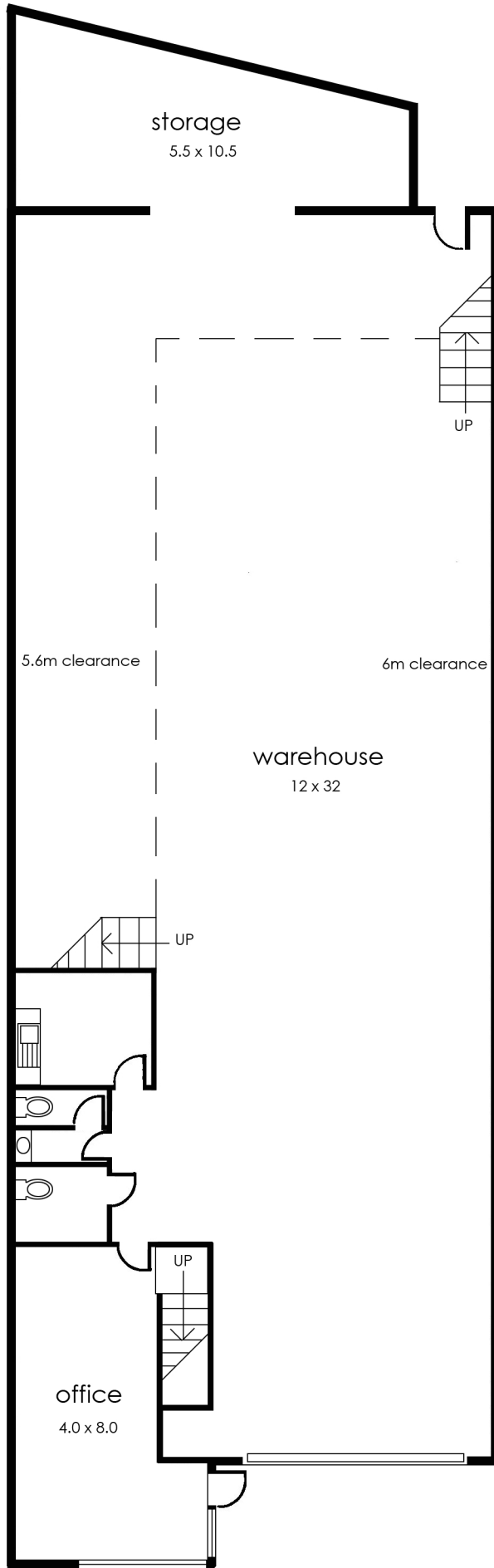
GROUND FLOOR
