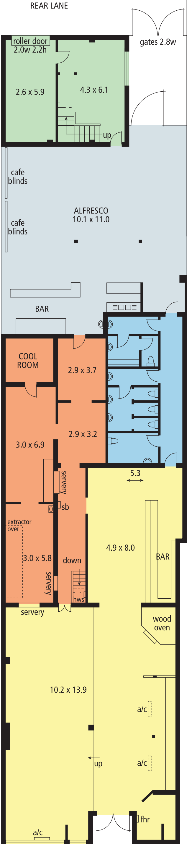
GROUND FLOOR
