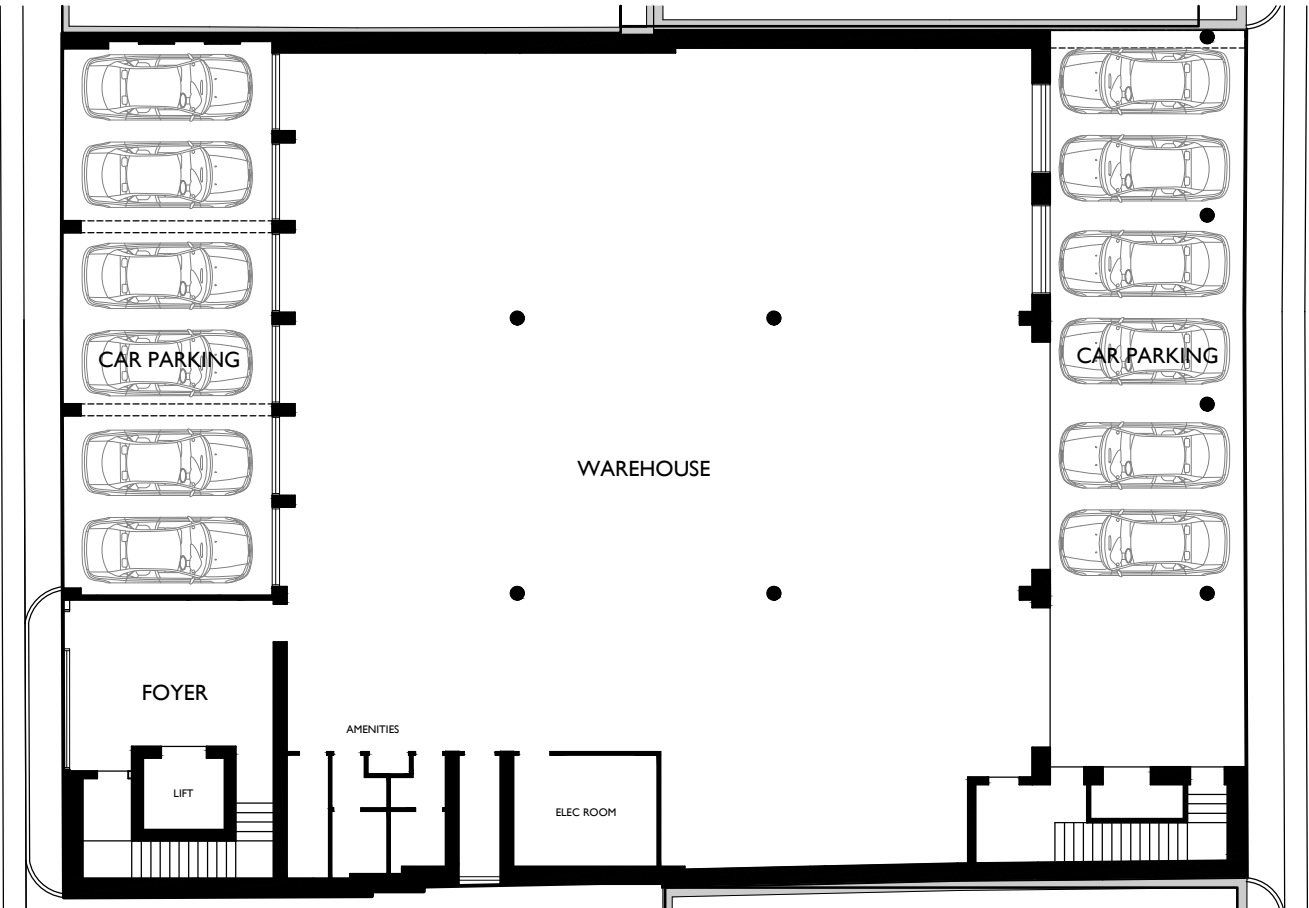
GROUND FLOOR
