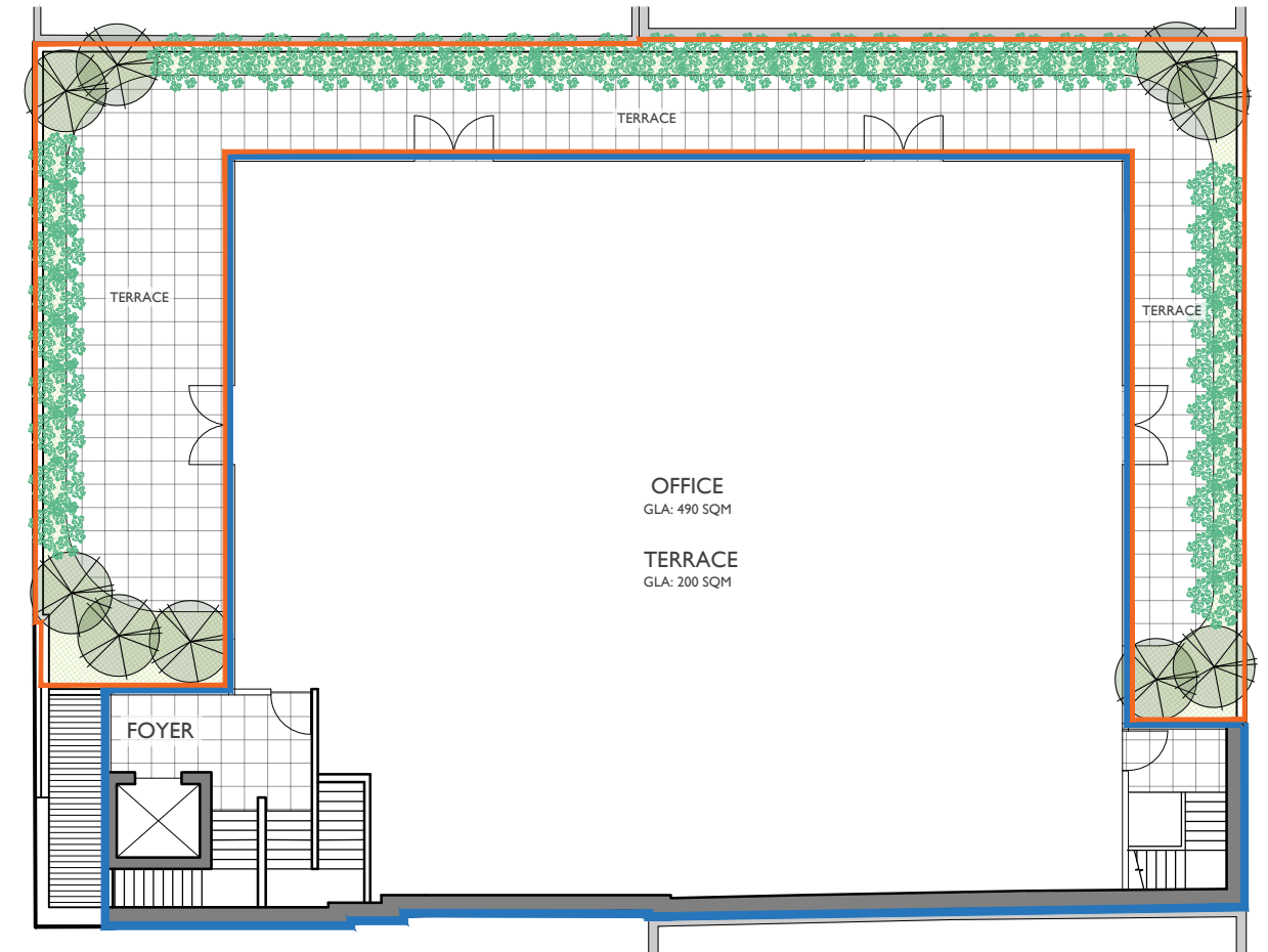
THIRD FLOOR
