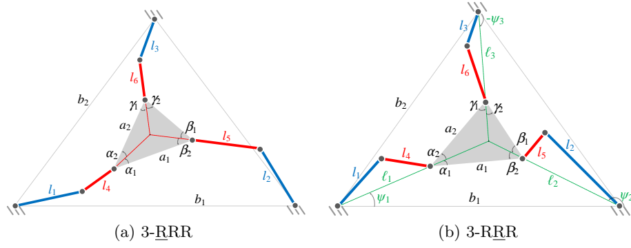
Fig. 4: 3-RRR input singularities
