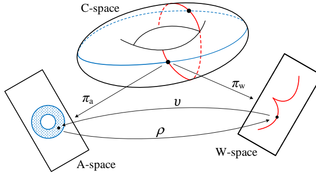
Fig. 1: Kinematic mappings and the C-space
