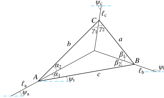
Fig. 5: Ceva's theorem
