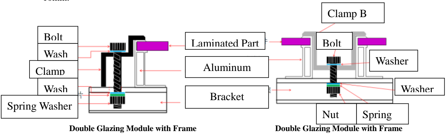
Clamp installation guideline
