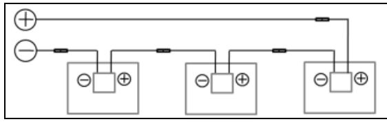
Series Connection
