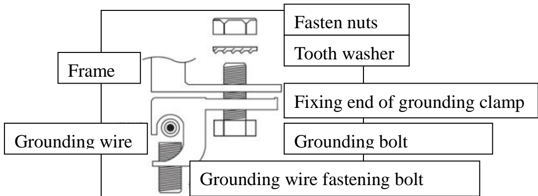
Figure 7 Install Method
