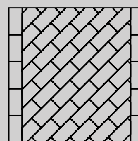
45° Stretcher Bond with flat header course
