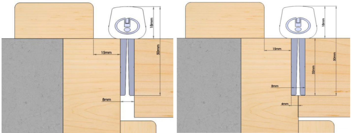
Non Rebated Layout
